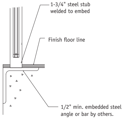
Top mounting
