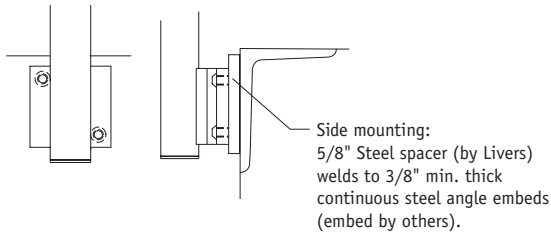
Side mounting
