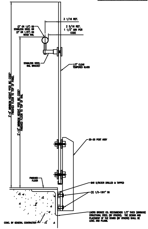
SECTION SCALE 3/4"=1'-0"
