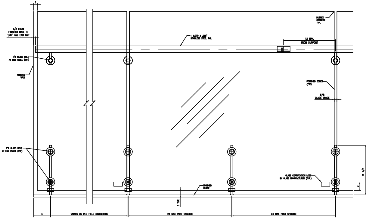
ELEVATION SCALE 3/4"=1'-0"
