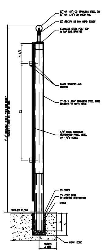
SECTION SCALE 3/4"=1'-0"
