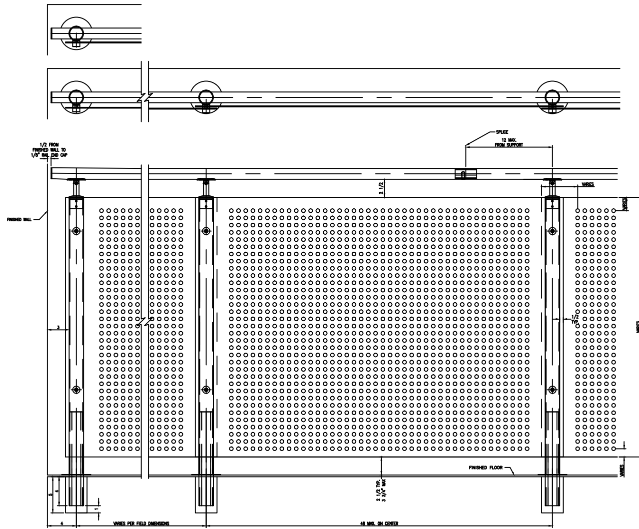
ELEVATION SCALE 3/4"=1'-0"
