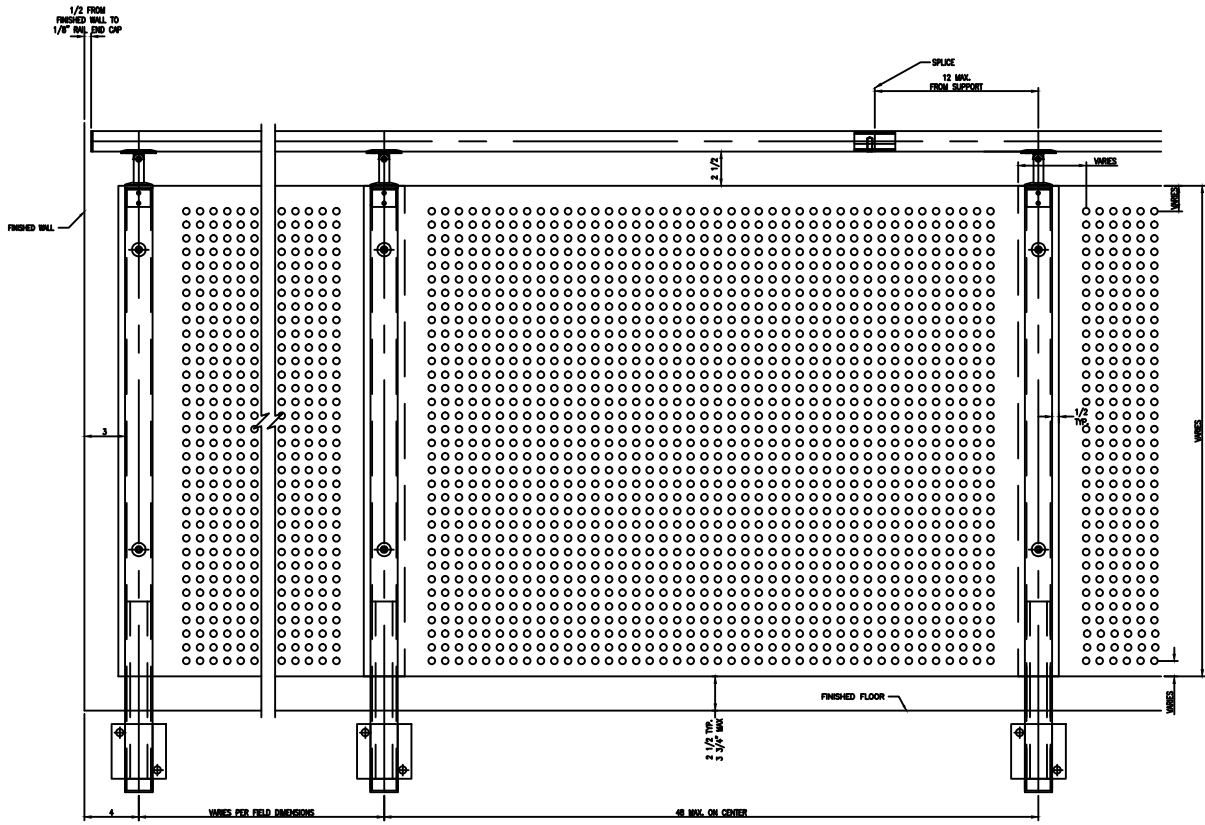
ELEVATION SCALE 3/4"=1'-0"
