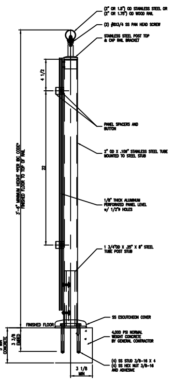
SECTION SCALE 3/4\"/>
