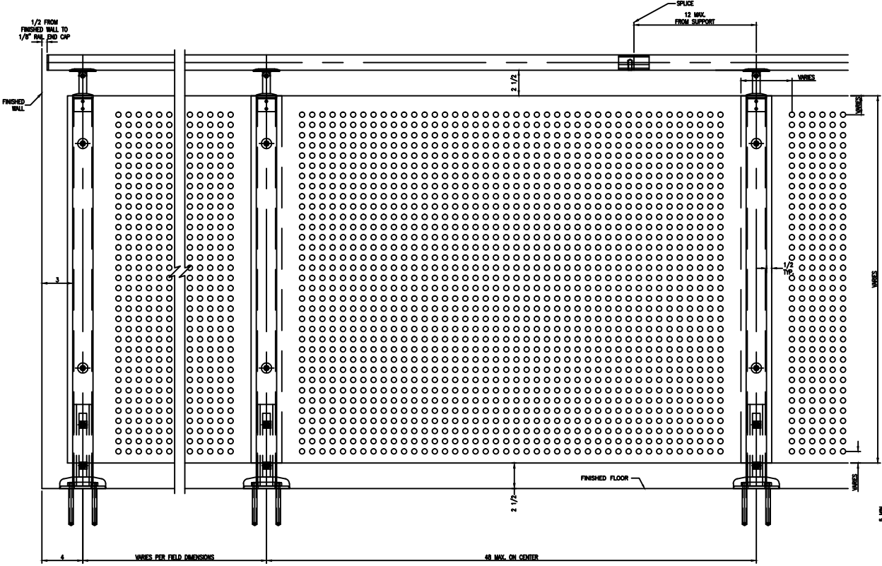
ELEVATION SCALE 3/4\"/>
