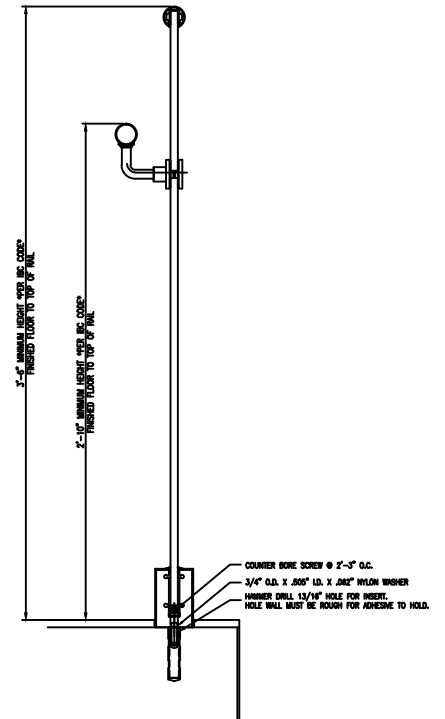
SECTION SCALE 3/4"=1'-0"
